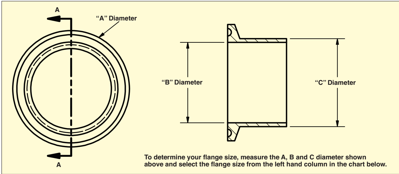
TRI-GRIP® PROCESS MOUNTING FLANGE DIMENSIONS
